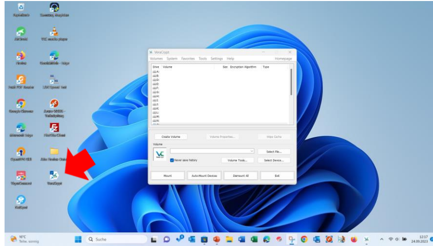
1. VeraCrypt starten
